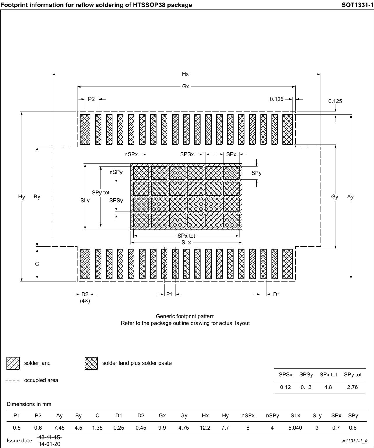
Fig 26. PCB footprint for SOT1331-1 (HTSSOP38); reflow soldering
